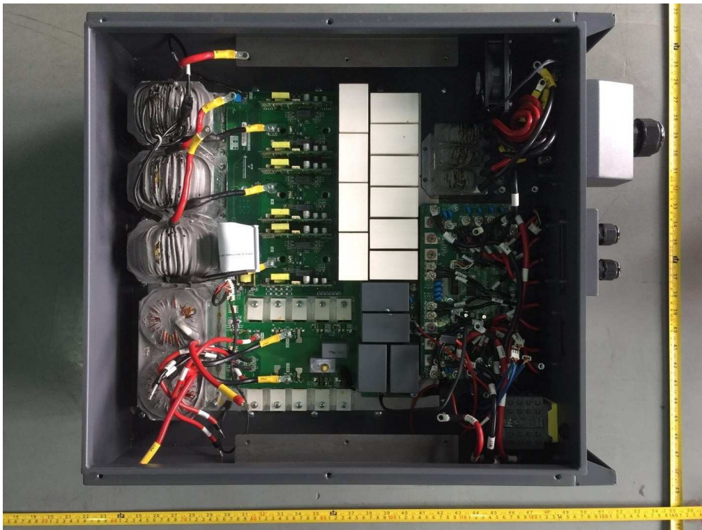
Internal view: EVVO 30000TLG23P, EVVO 33000TLG23P
